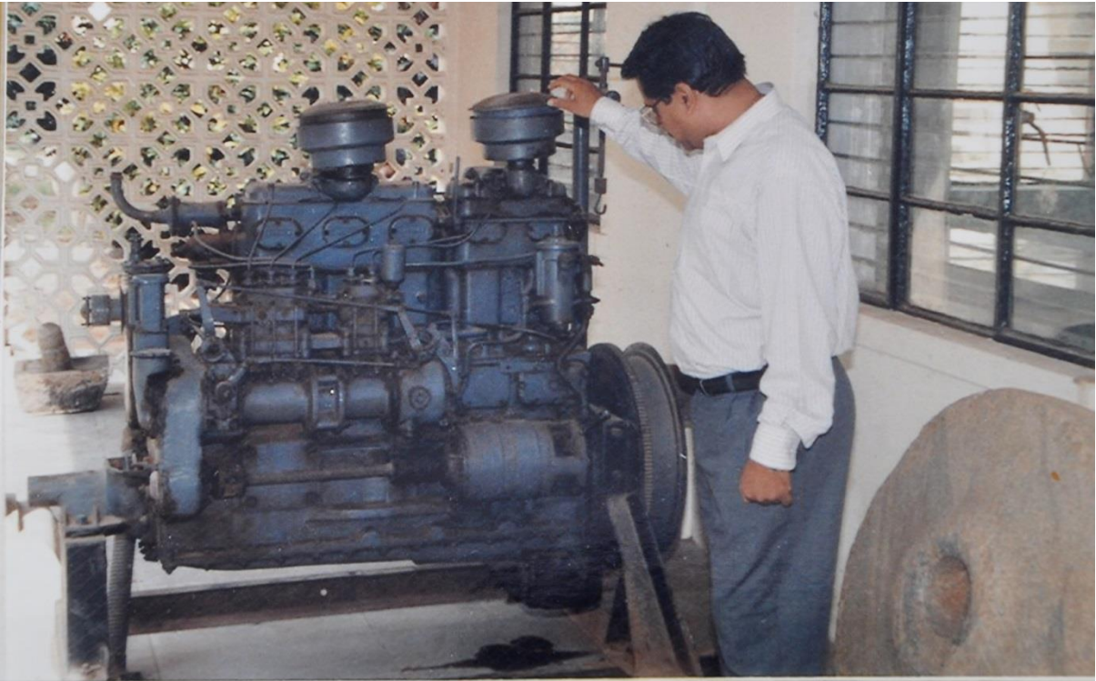
Explicating 5 cylinder military vehicle engine of 1940s
